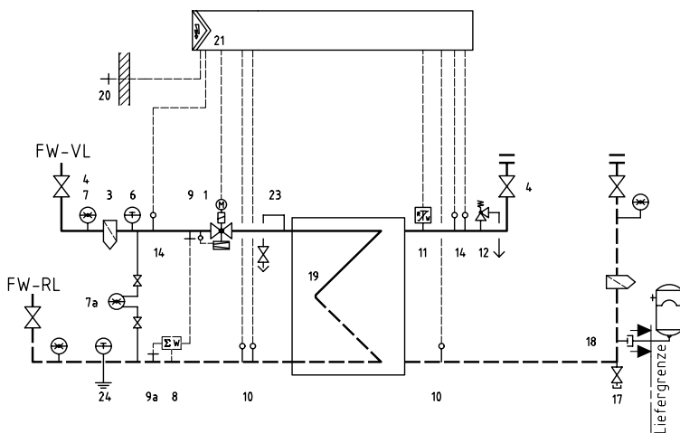
Hydraulic diagram
