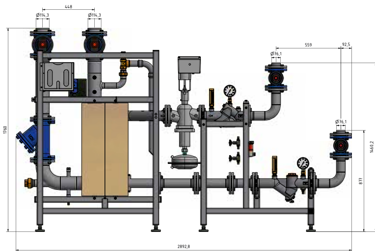
Technicle drawing
