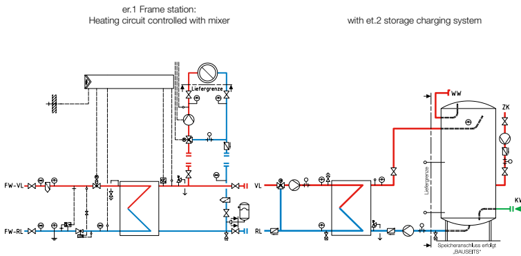
Hydraulic diagram of the station
