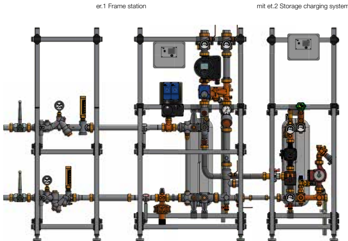
Technical drawing of the station
